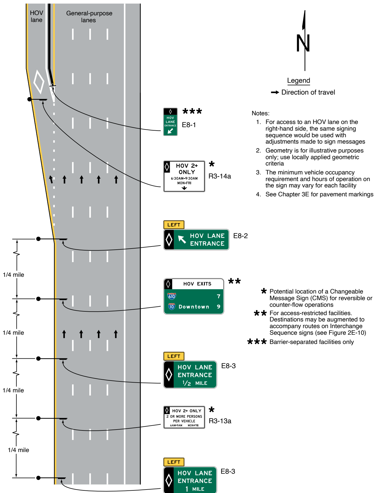
Figure 2G-9. Example of Signing for an Entrance to Access-Restricted HOV Lanes
